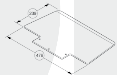
Toe plate GS-NG 476 x 239 x 7 mm, for packages (e.g. beverage cans), article no. 930 084
