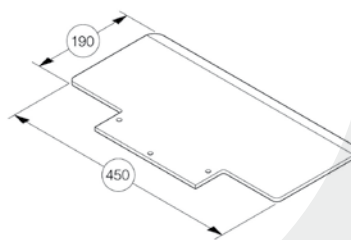
Toe plate DS-NG 450 x 190 x 7 mm, suitable for packages, article no. 930 085
