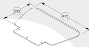
Toe plate V 413 x 233 x 5 mm, toe plate for transporting oxygen cylinders, etc., article no. 930 001
