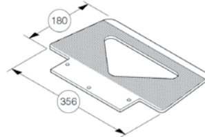
Toe plate WL 356 x 180 x 7 mm, for white goods, refilling vending machines etc., article no. 930 018
