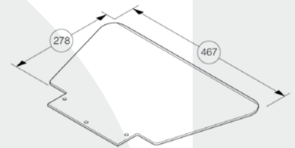
Toe plate LH 467 x 278 x 5 mm, same as toe plate V but larger, article no. 930 002
