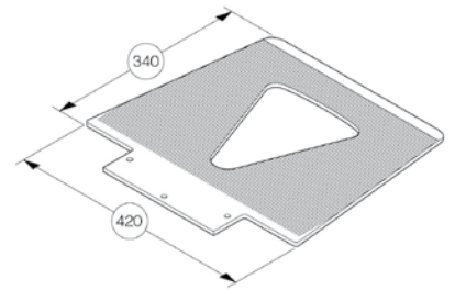
Toe plate G 420 x 340 x 7 mm, for large packages, article no. 930 003
