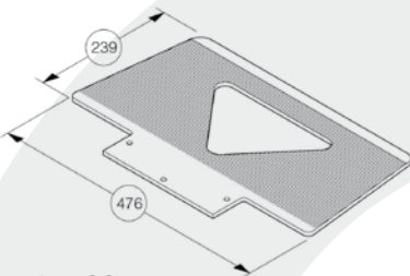
Toe plate GS 476 x 239 x 7 mm, as used in the beverages industry; wide enough for safe transport of kegs and crates - no straps required, article no. 930 030
