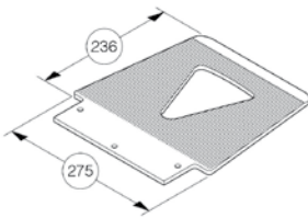
Toe plate Standard 275 x 236 x 7 mm, with grooves to prevent load slipping sideways, article no. 030 025
